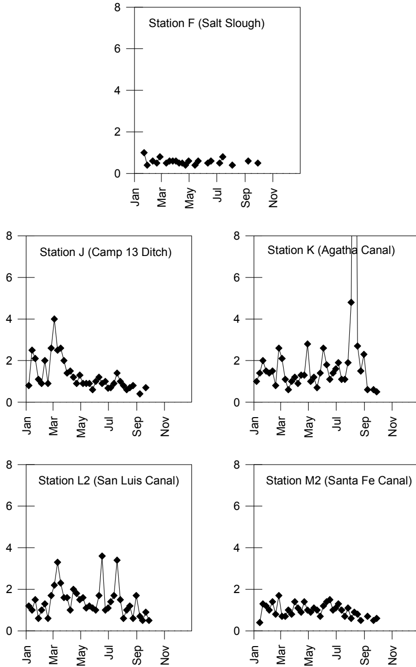
Figure 6. Selenium concentration ( \mu\text{g/L} ) at Station F (Salt Slough) and in wetland water supply channels at Station J, K, L2, and Station M2. Data from weekly samples.
