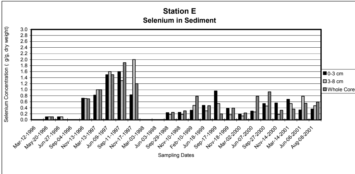
Figure 18. Selenium concentrations in sediment at Stations E (Mud Slough at Highway 140) and F (Salt Slough). Samples not tested at Station E for March 1996, September 1996, March 1998, and June 1998 and at Station F for March 1996. Other missing bars indicate concentrations were below limits of detection.
