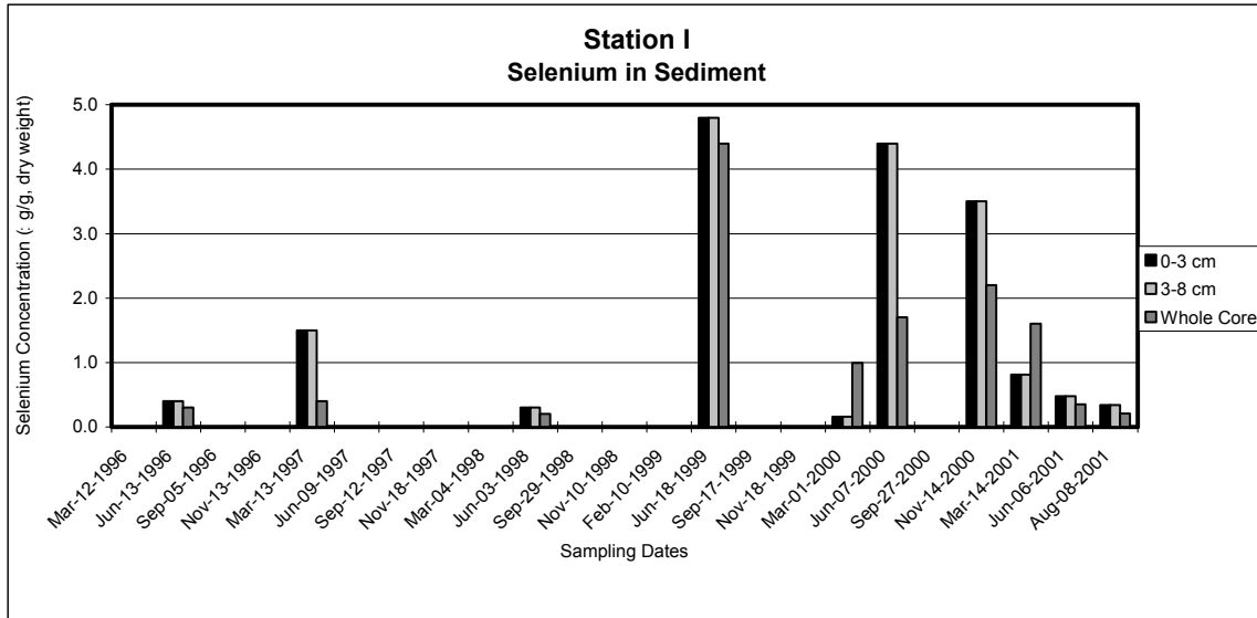
Figure 19. Selenium concentrations in sediment at Station I (Mud Slough back water annual site). Samples with missing bars were not tested. June 2001 samples were taken at Station I2.
