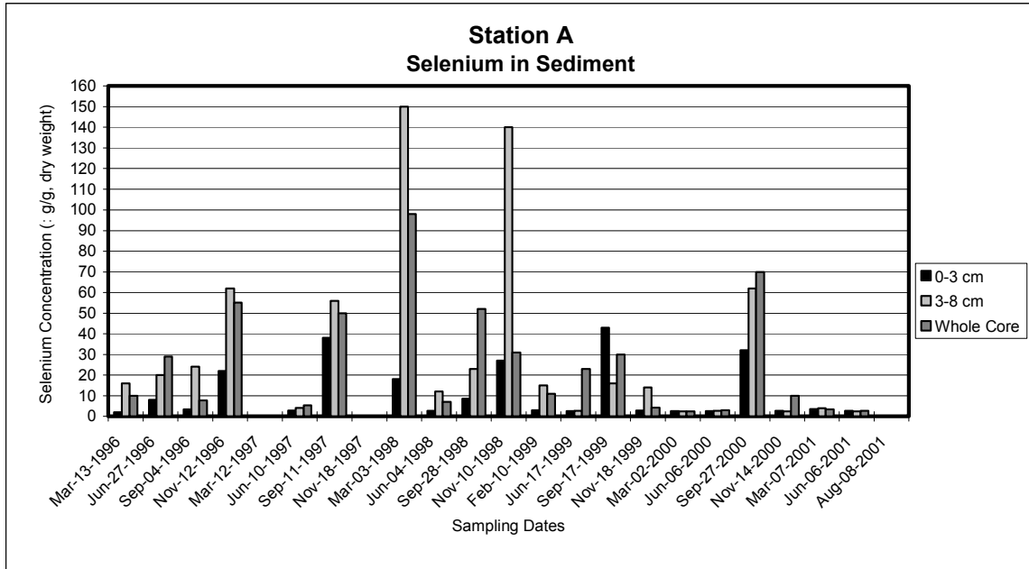
Figure 16. Selenium concentrations in sediment at Stations A (inlet to San Luis Drain) and B (discharge from San Luis Drain). Samples were not tested from Station A on March 1997, November 1997, and August 2001. Station B samples from March 1996, June 2000, November 2000, and June and August 2001 were also not tested. Concentration in whole core sample at Station B in June 1997 was 0.11 \mu\text{g/g} dry weight.
