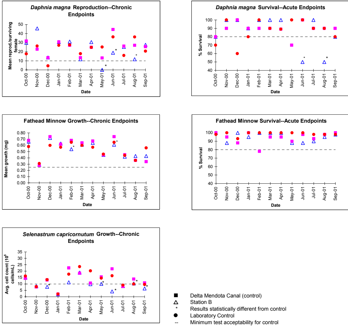
Figure 12. Comparison of toxicity test results from Station B with results from the Delta Mendota Canal reference location. The different tests are described in the text.
