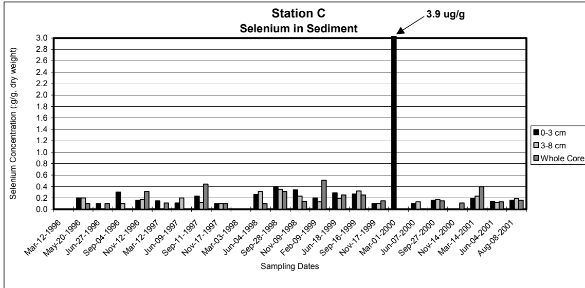
Figure 17. Selenium concentrations in sediment at sites C (Mud Slough upstream of the GBP discharge) and D (Mud Slough downstream of the GBP discharge). Samples not tested at Stations C and D for March 1996 and March 1998. Other missing bars indicate concentrations were below limits of detection.
