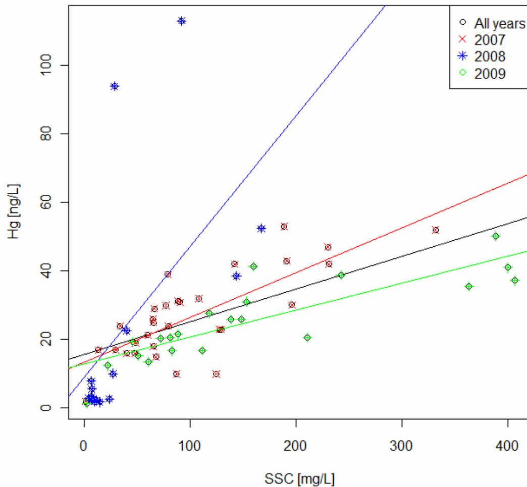
Figure A.1. SSC: Hg relationships at Zone 4 Line A. The mean slope estimate for 2007 – 2009 were 0.13, 0.38, and 0.08, respectively. The mean slope of all three years was 0.19.
