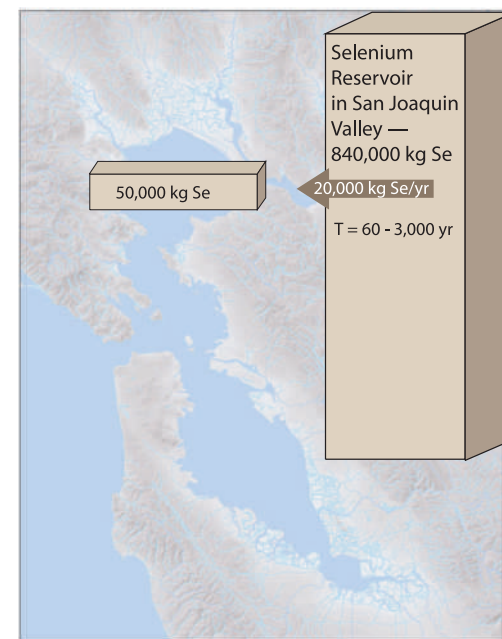
Figure 3. A major limitation of all the conceptual models has been inadequate knowledge of the quantity of contaminant in the soil of Bay watersheds, and the potential for this material to reach the Bay. This Figure depicts the soil reservoir of selenium compared to its loading and reservoirs in the Bay (modified from Abu-Saba, 2004). For many priority contaminants, the amount of material stored in watersheds with the potential to wash off into the Bay presents the biggest challenge to the continued recovery of the ecosystem. In general, the size of the soil reservoir and its potential to reach the Bay are very poorly understood.
