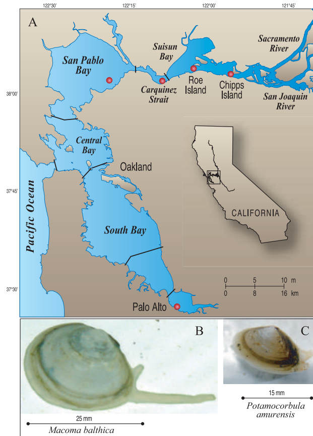
Figure 1. San Francisco Bay is a complex and variable ecosystem. A) Map of San Francisco Bay with four sites in the northern reach of the Bay (Chippis Island, Roe Island, Carquinez Strait, and San Pablo Bay) and one site (Palo Alto) in the southern portion. B) Macoma balthica , the deposit feeding clam collected in the mudflat at the Palo Alto site. C) Potamocorbula amurensis , the suspension feeding clam collected in the channel at the northern reach sites.
