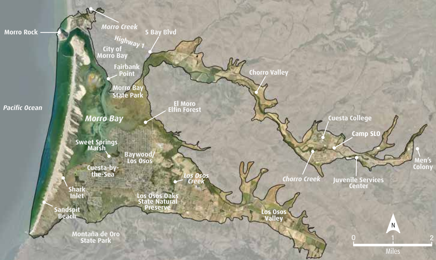
Figure 1. The project study area , which includes the Morro Bay Estuary, Morro Rock, the sandspit, the young alluvial deposits of Chorro Valley and Los Osos Valley, and the old eolian deposits in the Baywood/Los Osos area. The study area encompasses 59 km 2 (23 mi 2 ) of the Morro Bay Watershed (197 km 2 or 76 mi 2 ).
