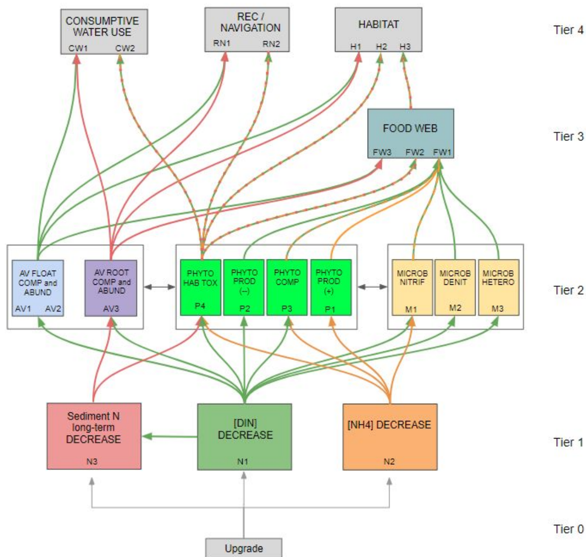
Figure 2. Plausible mechanistic pathways developed for the conceptual framework. Arrows between tiers indicate plausible pathways that have been hypothesized or proposed in Bay-Delta scientific literature or management considerations. Arrow colors extending from T2 to T3 or T4 indicate whether the continued path is related originally to N1 (green), N2 (orange), or both. \leftrightarrow denotes interactions/feedbacks between T2 responses, P \leftrightarrow M , AV \leftrightarrow P , and AV \leftrightarrow M . See Table 1 for a more detailed description of the potential responses (Figure prepared for Senn et al. in prep ).
