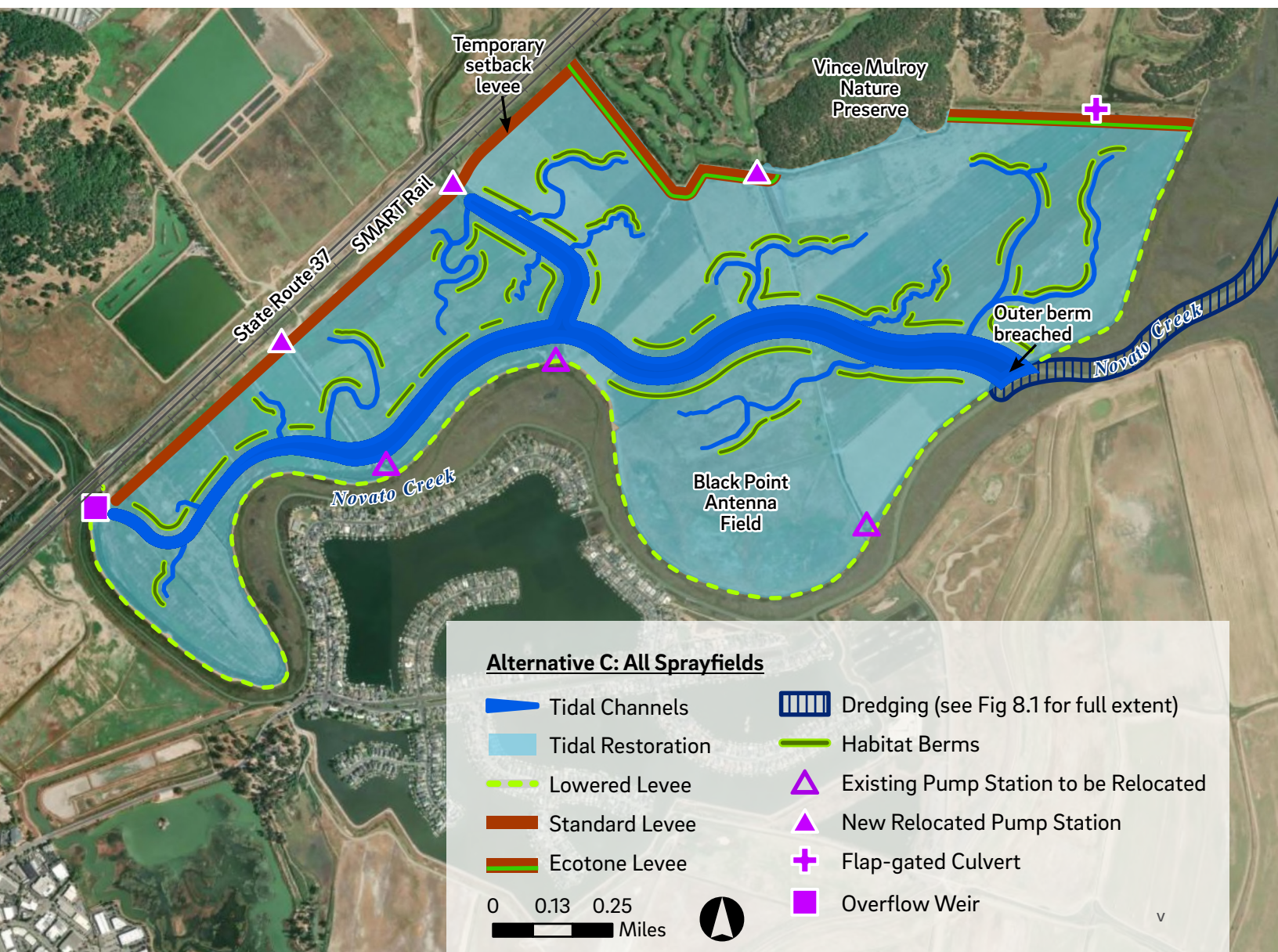
Figure ES-2. Alternative C: All Sprayfields emerged as the preferred first project to pursue due to its cost efficiency, large restored area, and flood reduction benefits.
